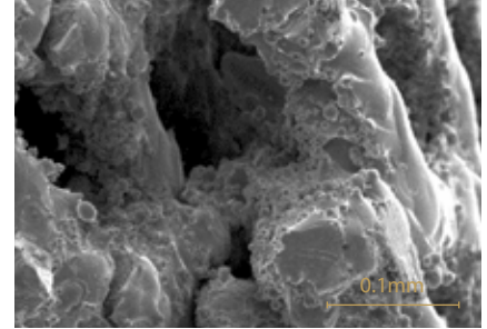
Nano pores
