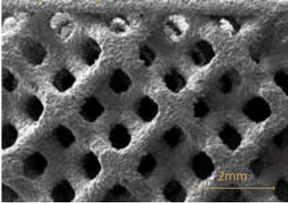
Macro pores
