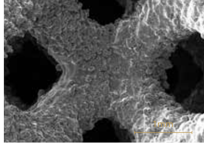
Micro pores
